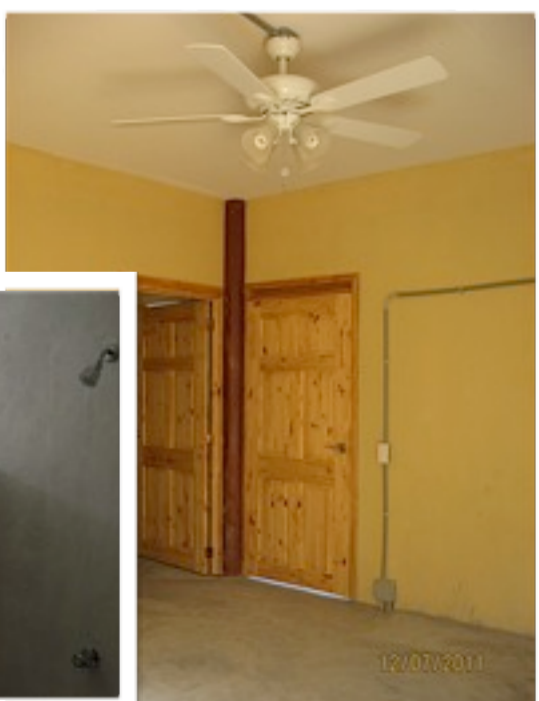
Septic field and tank for plumbing were installed to serve six bathrooms, 2 shower rooms, and sinks in each consultation room. Glass sliding windows, fans and lights are installed.
